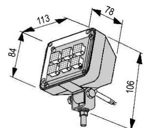
LD116 Advance dimensions (mm) Swivel mounting kit.
