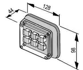
LD116 Advance dimensions (mm) Surface mounting kit.
